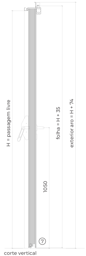
corte vertical
